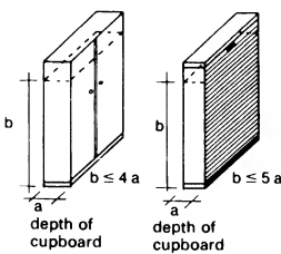
④ Relationship between depth and height of cupboards
